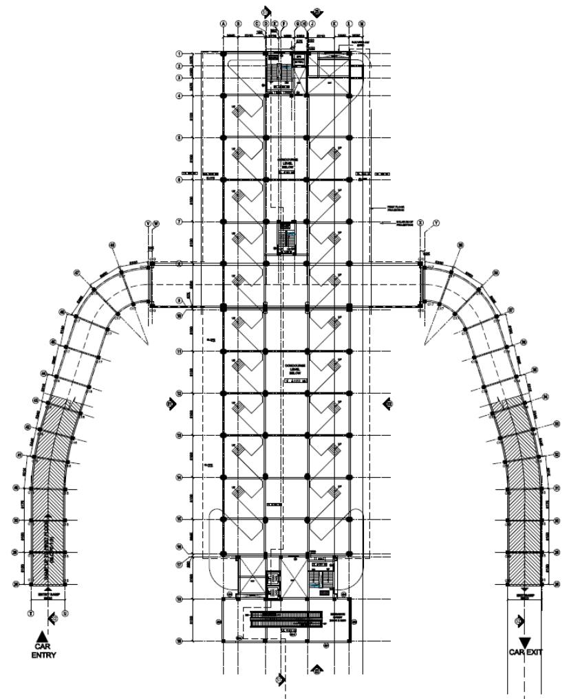
FLOOR PLAN at Lvl +4350
