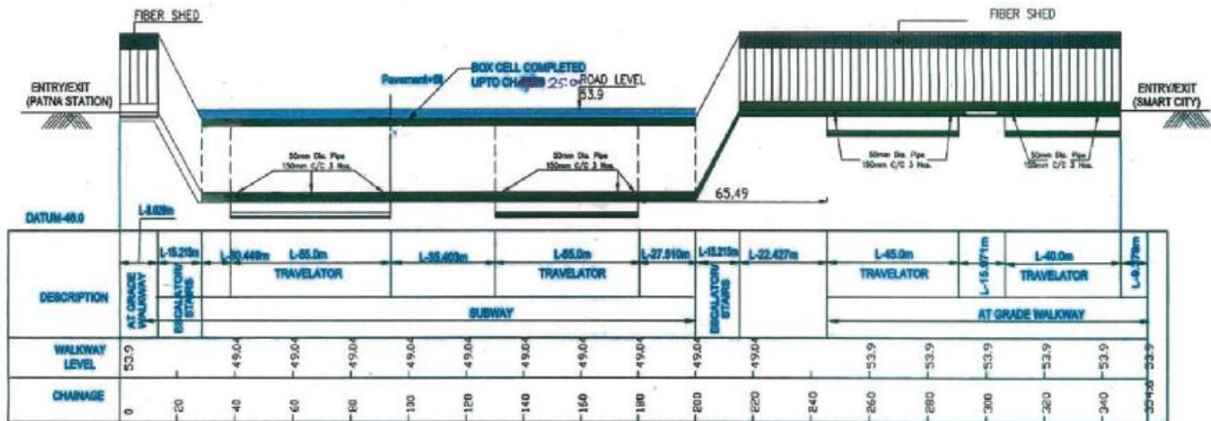
SECTIONAL ELEVATION OF SUBWAY
