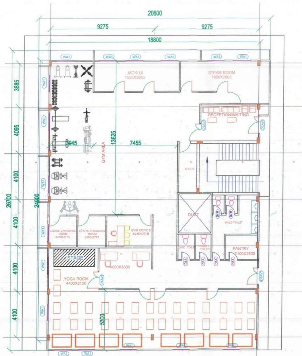
GYM DETAILS
